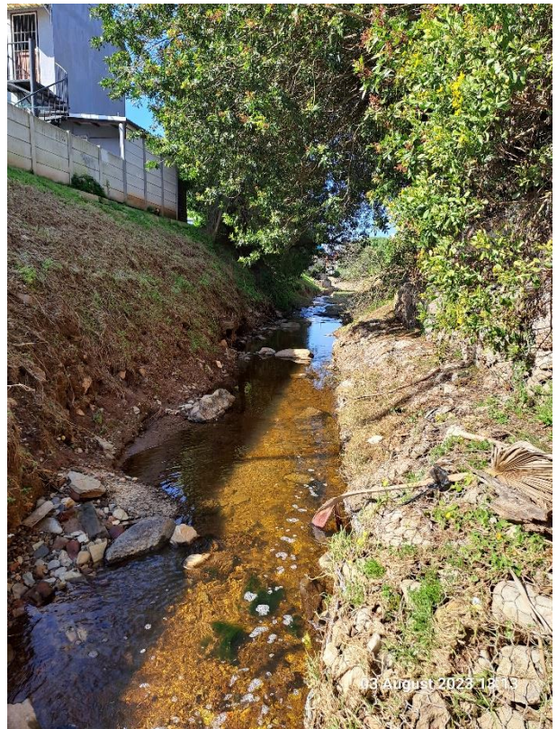
Current state of the channel and side slopes with ad-hoc slope protection
